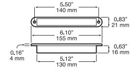
Optional B388-09X chrome bracket
