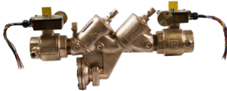
SLOW CLOSE WITH MONITOR SWITCHES T2ST OPTION (1-1/2" AND 2" ONLY) SEE SS1397 FOR DIMENSIONS
