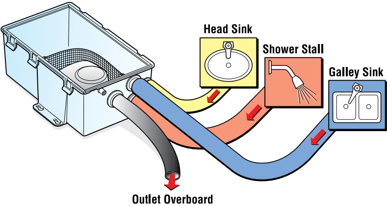
Outlet Overboard
