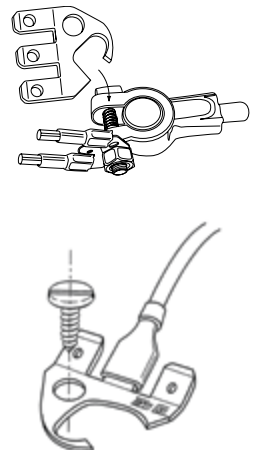
#30703 Kit - 1 Tap, 3 Slip-On Terminals #30703-7 - Tap Only
