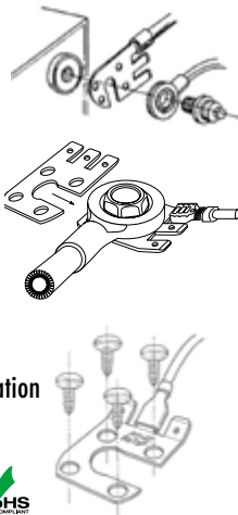
#30703 Kit - 1 Tap, 3 Slip-On Terminals #30703-7 - Tap Only
