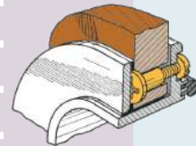
FLUSH MOUNT BARREL NUT PORT INSTALLATION
