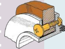
STANDARD BARREL NUT PORT INSTALLATION
