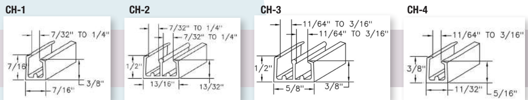
ALL RIGID WINDOW CHANNEL- MODEL# CH-1, CH-2, CH-2BR, CH-2B, CH-3, CH-3BR, CH-4
