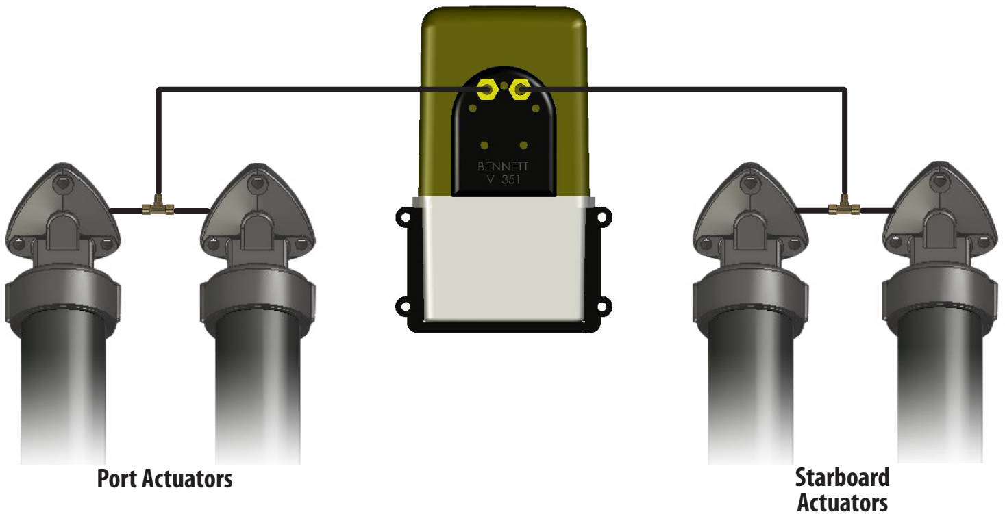
Tubing Diagram for Dual Actuator System
