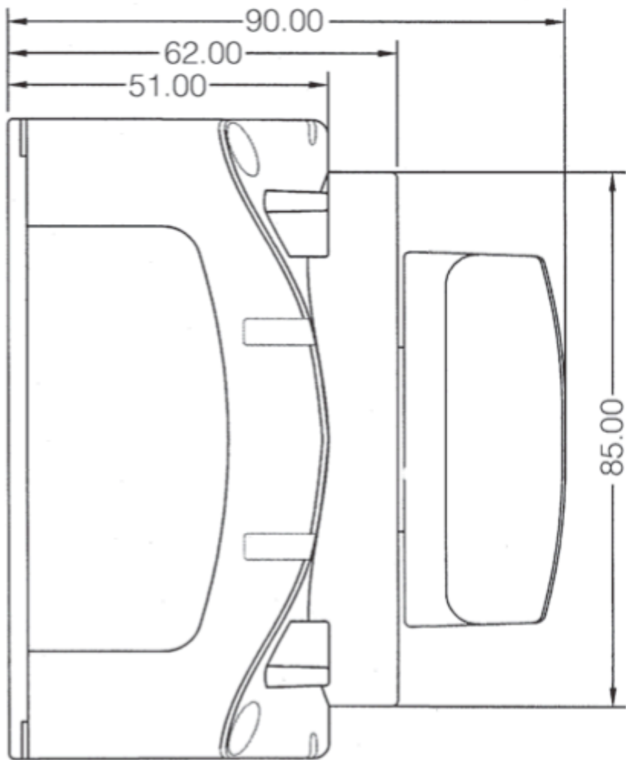
Dimensions for 72I Switch
