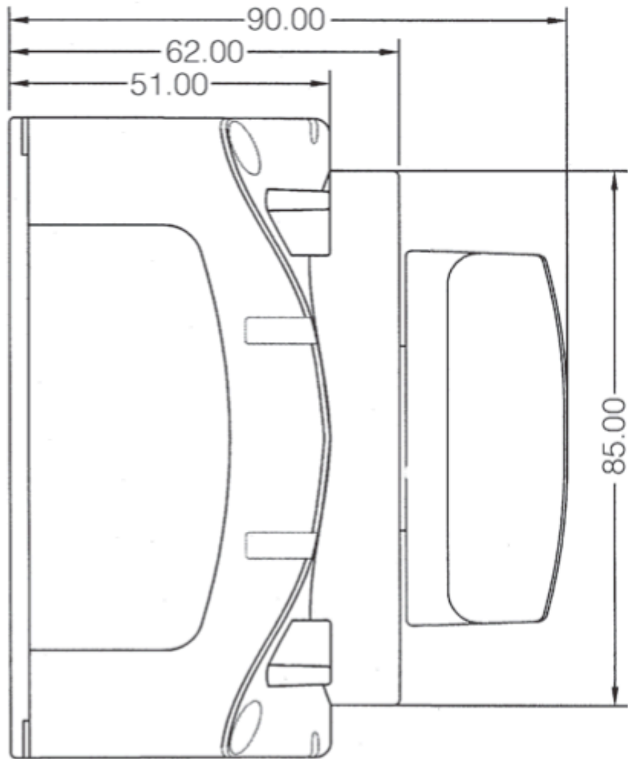
Dimensions for 721 Switch
