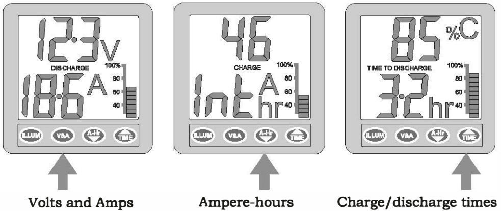
Figure 2 - Operating modes
