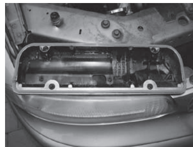
PermaDry® gasket installed dry
