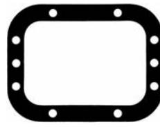
55377 9-1/4" x 7" 8-Bolt
