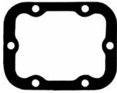
55372 6-1/4" x 5" 6-Bolt
