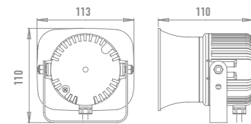
LOUDSPEAKER - NSC
