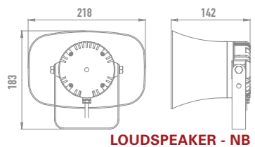
LOUDSPEAKER - NB
