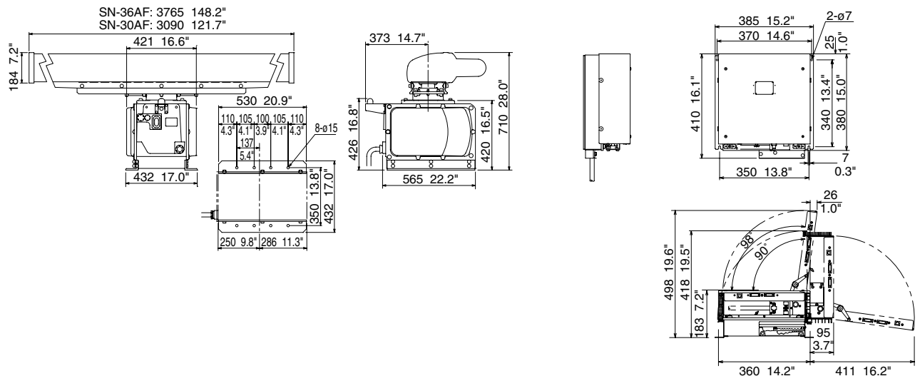
10 ft S-band Antenna
