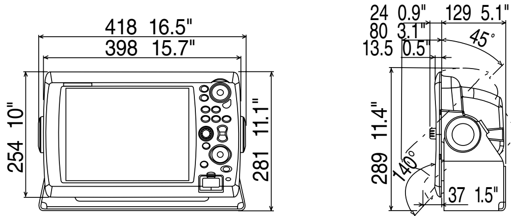
Multi Function Display (Table-top Mount) MFD12
