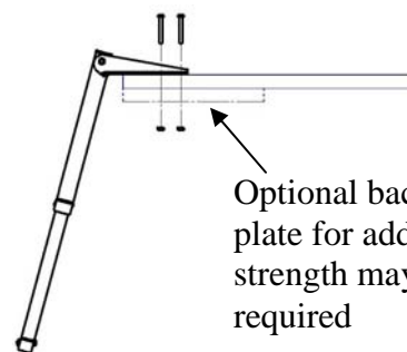
Figure 1 FASTENER SUGGESTION
