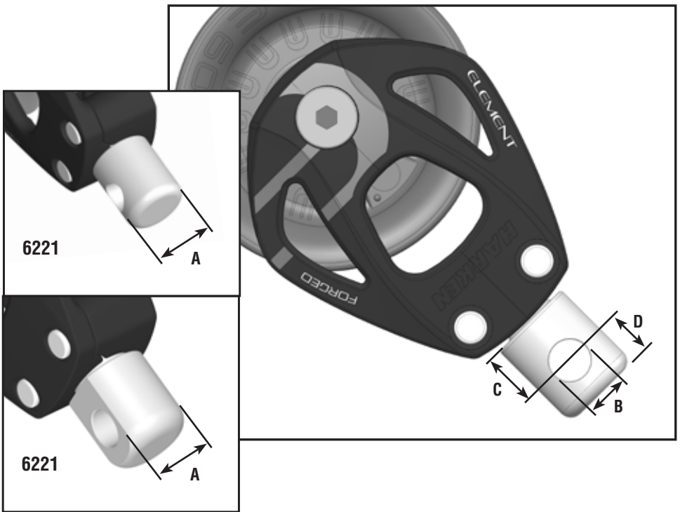
Forkhead fitting
