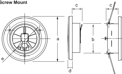
Screw Mount
