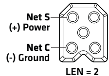
NMEA 2000® Port [optional]
