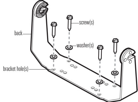
Installing the Gimbal Bracket
