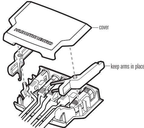
Assembling the Cable Tray
