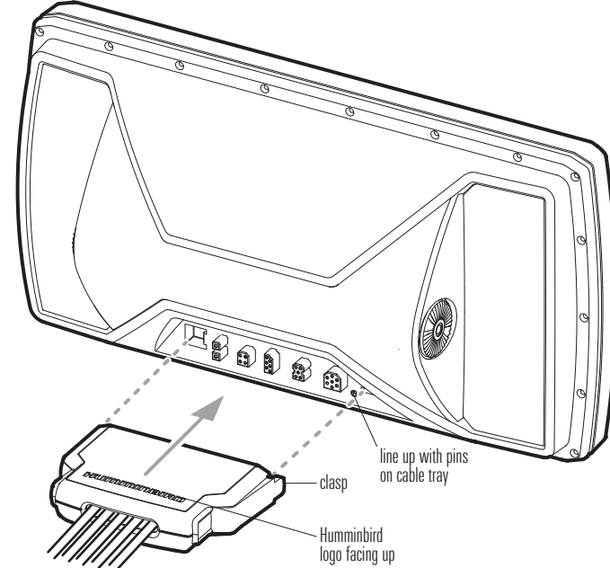
Connecting the Cable Tray to the Control Head
