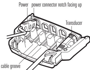
Inserting the Cable Connectors into the Cable Tray
