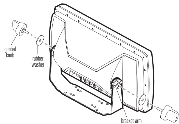
Assembling the Control Head and Bracket
