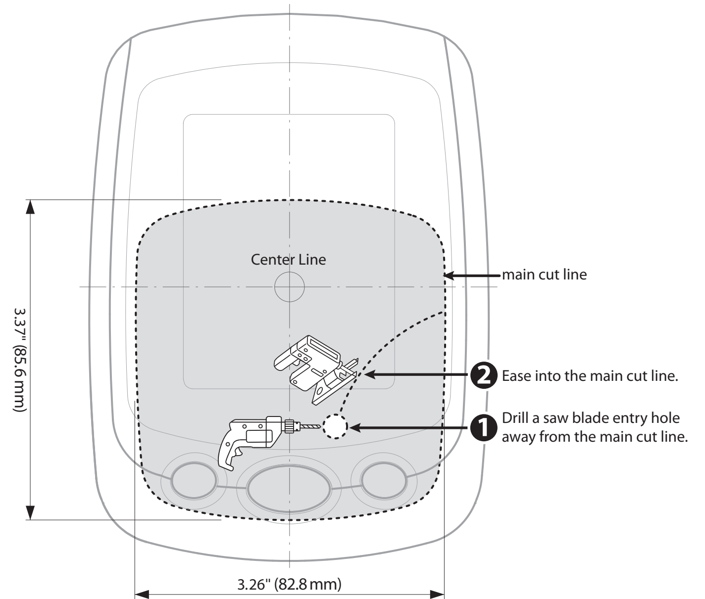
Template for 3-Button PiranhaMAX Models
