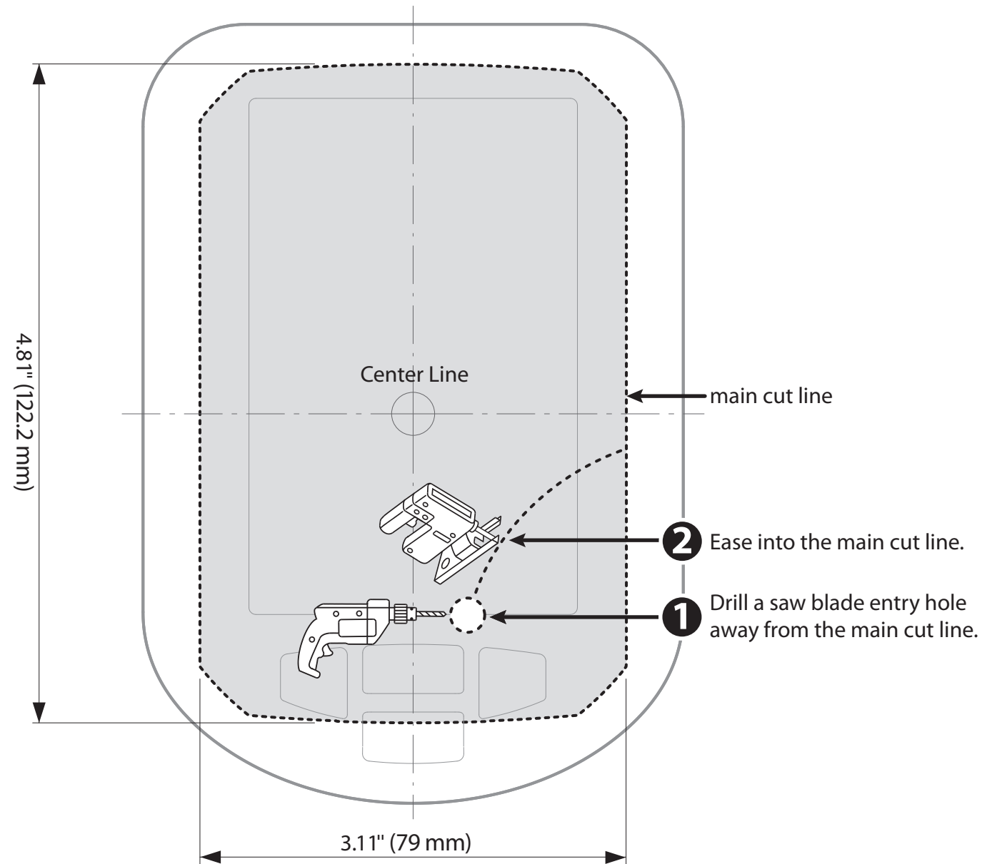
Template for 4-Button PiranhaMAX Models
