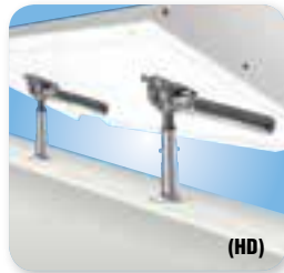
"Dual" Locking Surface Deck Socket with "LevelLock" Mount T10-522
