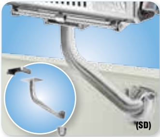
Vertical Surface Side Mount T10-344
