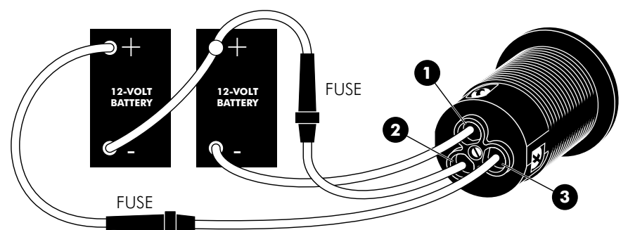
DUAL VOLTAGE CONFIGURATION
