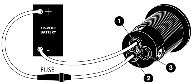
12V CONFIGURATION
