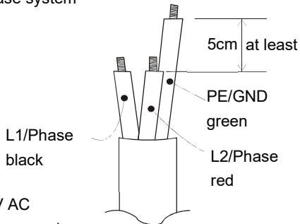
USA 120V AC Single phase system
