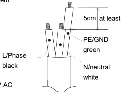
Europe 230V AC Single phase system
