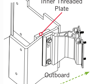
2e Inner Threaded Plate
