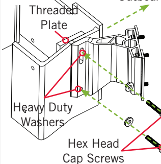
2c Inner Threaded Plate
