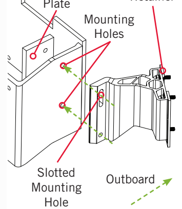
1b Inner Threaded Plate
