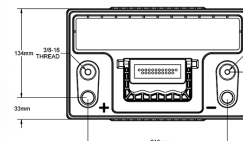
ODP-AGM34M LEFT POSITIVE DUAL TERMINALS (SAE & STUD)
