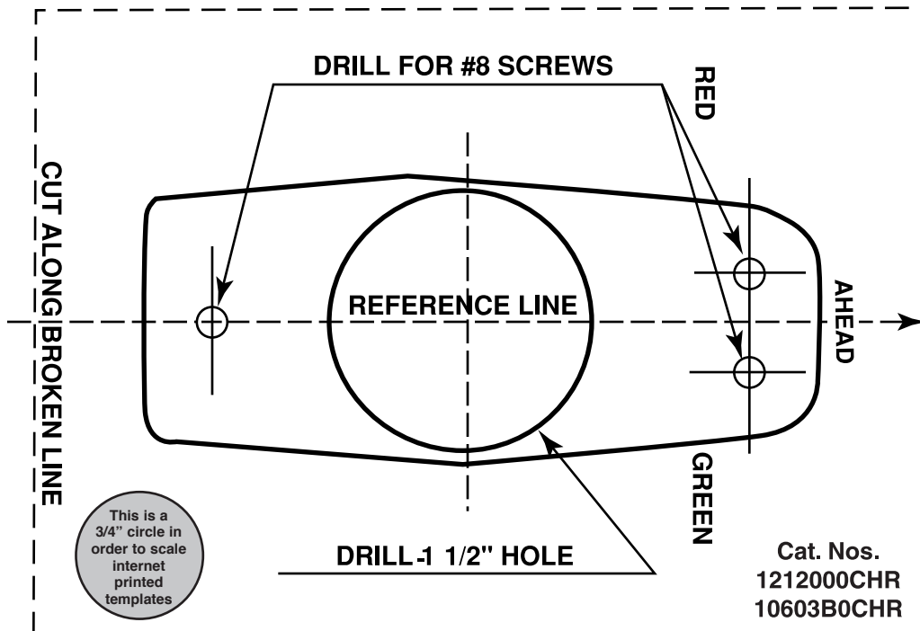
Fig. 1212 MOUNTING TEMPLATE
