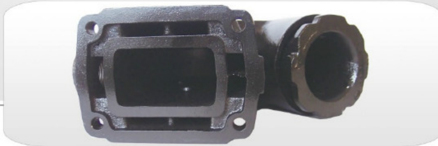
T-20921 Riser 3-1/2" exhaust outlet, 60° down angle, and tapped to accept 3/4" MPT hose barb.
