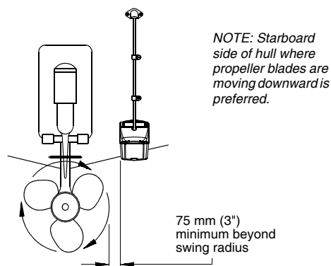
Figure 2. Mounting location on single drive boat
