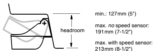
Figure 1. Headroom required on a stepped transom
