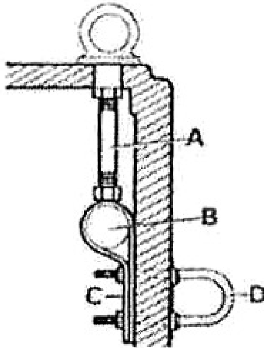
Stern Assembly
