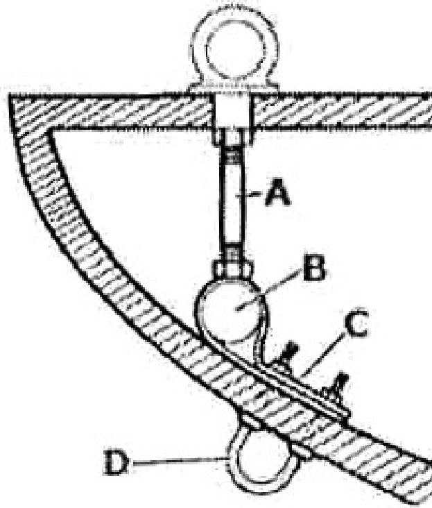
Bow Assembly
