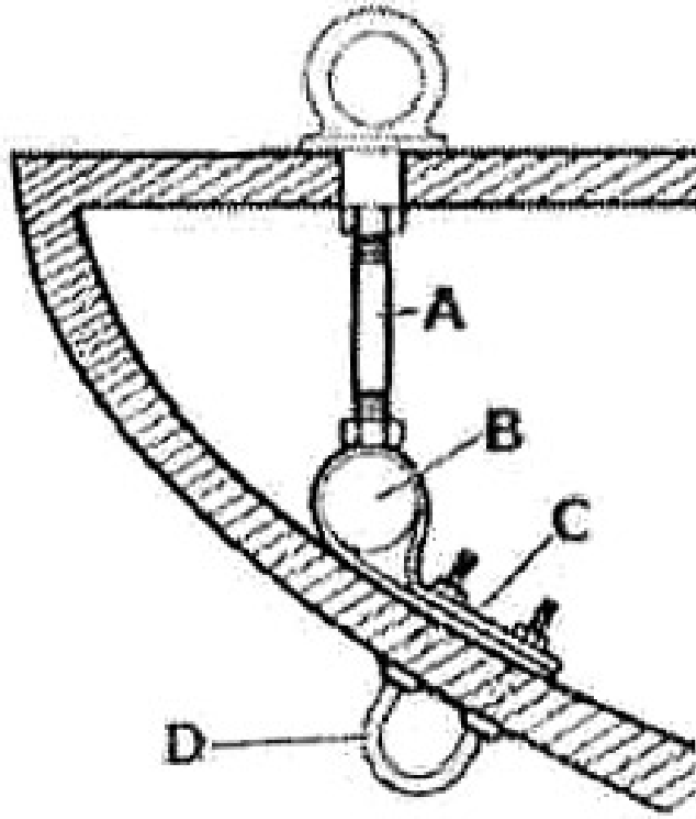
Bow Assembly
