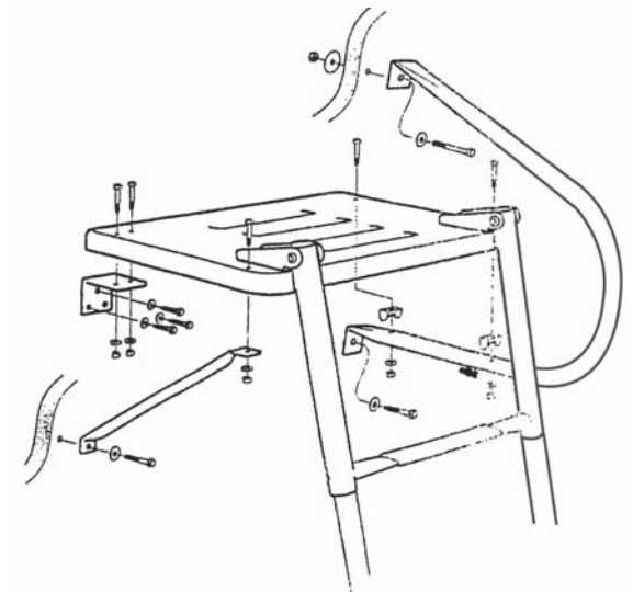
Figure 2 Outboard Application
