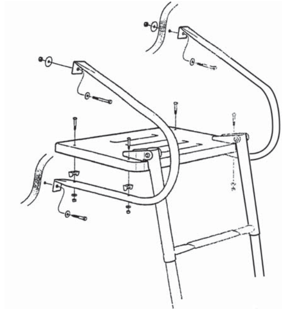
Figure 1 Inboard/Outboard
