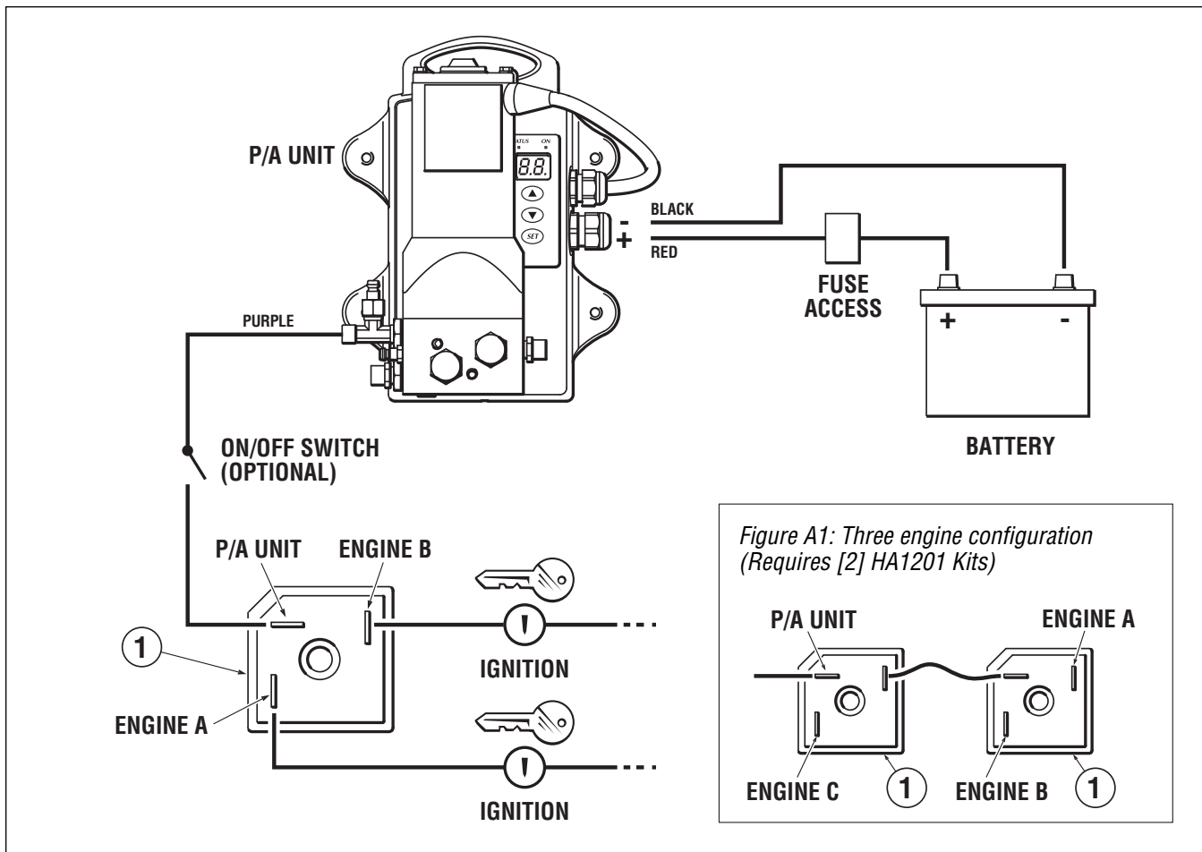
Figure A. Two engine configuration.
