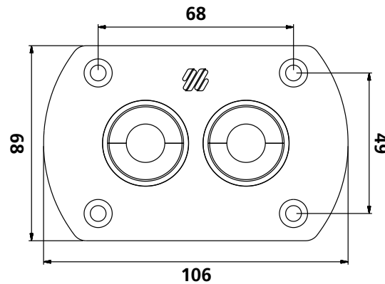
R8 DIMENSIONS
