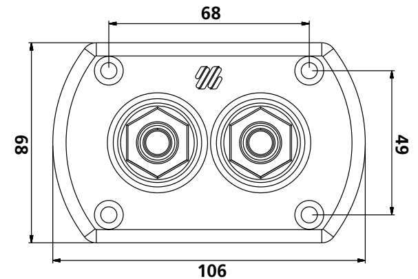
R9 DIMENSIONS
