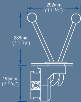
BP4410 Thru Deck/Bulkhead Side View
