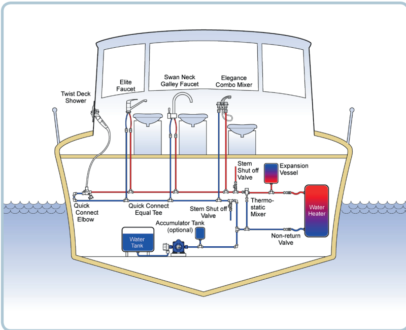
Typical Installation
