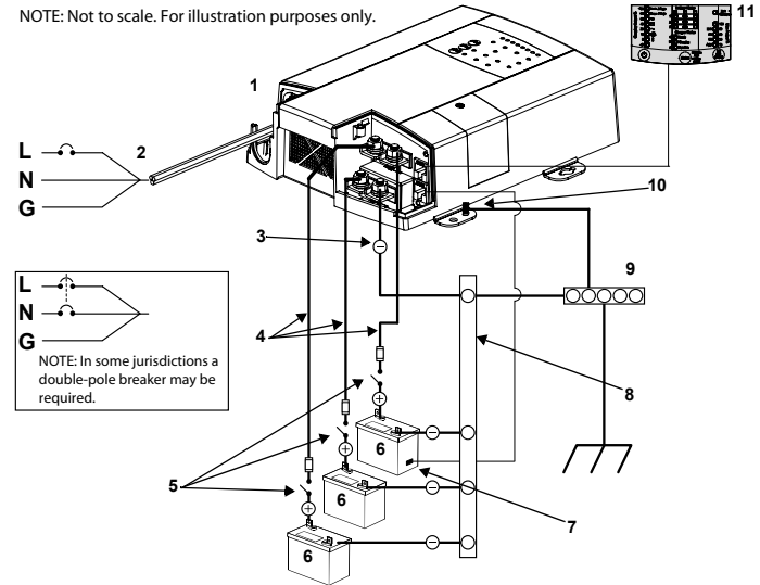
Figure 4 Configuration for Normal Loads
